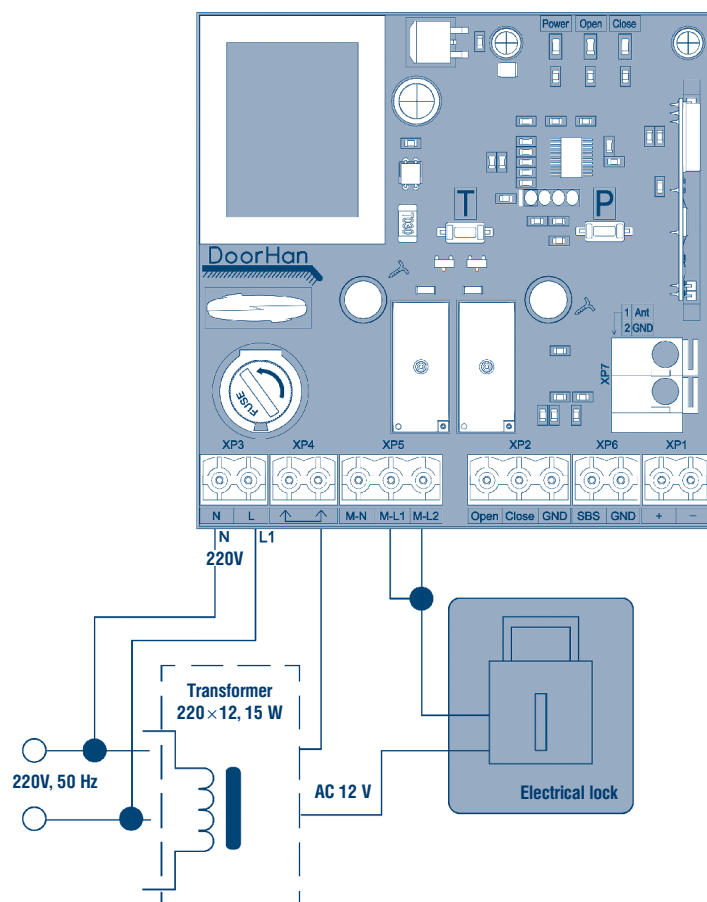
Fig. 3. Connection of electrical lock
